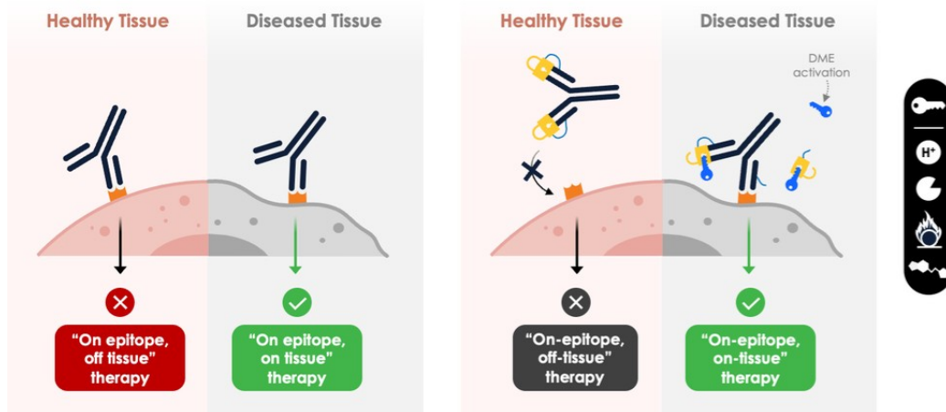
Figure 5: Mechanism of ShieldTx, iBio's masking technology to create conditionally activated antibodies
